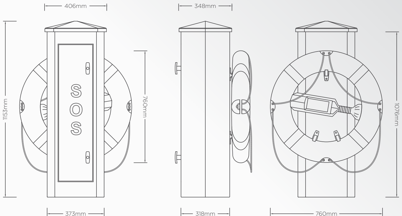
Hex SOS pedestal:
